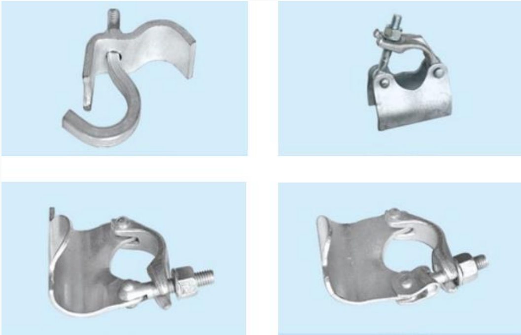
Putlog coupler
